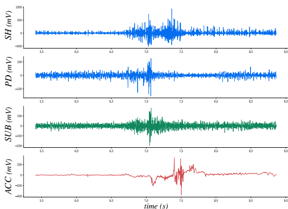
Figure 3: Raw signals of a saliva swallowing. SH: stylohyoid, PD: posterior digastric, SUB: submental, ACC: accelerometer. All signals provide distinguishable events. The burst of higher frequency in the ACC signal corresponds to the moment where the bolus goes through the upper esophageal sphincter.
